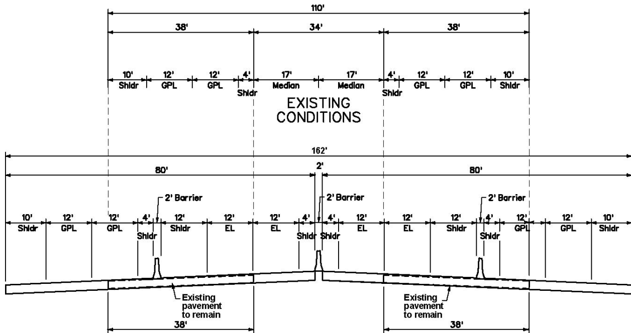
Figure 9.4 Proposed Typical Section
